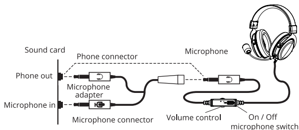
Fig. 2. Connection diagram
